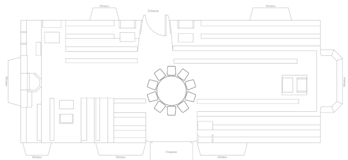
INNER LAYOUT 1no. 5' ROUND TABLE 10m
